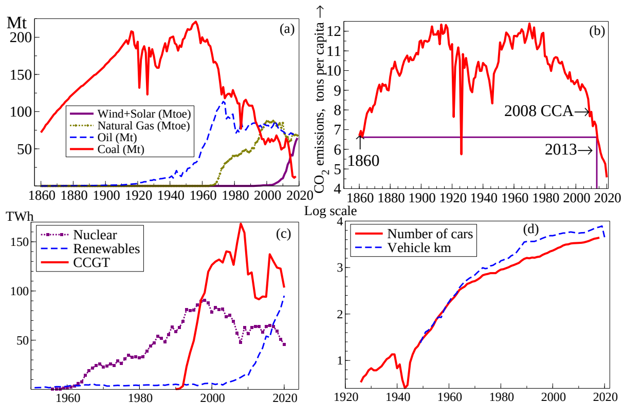
Figure 2: (a) UK coal (millions of tonnes, Mt), oil (Mt), natural gas (millions of tonnes of oil equivalent, Mtoe) and wind+solar (Mtoe), all to 2019; (b) UK territorial per capita CO 2 emissions (tons per annum) till 2020; (c) Main non-coal sources of UK domestically generated electricity (CCGT denotes Combined Cycle Gas Turbine); (d) Number of cars (in millions) and kilometers driven per annum (in billions) in the UK on a log scale, adjusted to match in 1949 when distance-travelled data start.
